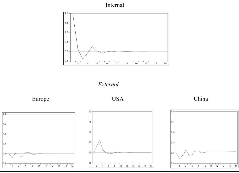
Figure 10: Impulse response function of the WAEMU to shocks from Côte d'Ivoire
