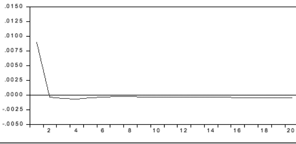
Figure 10: Impulse response function of the WAEMU to shocks from Côte d'Ivoire
